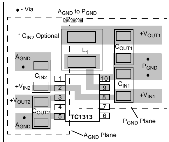
FIGURE 5-1: Component Placement, Fixed-Output 10-Pin MSOP.
