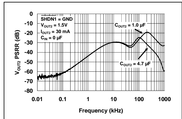
FIGURE 2-29: V_{OUT2} Power Supply Ripple Rejection vs. Frequency.
