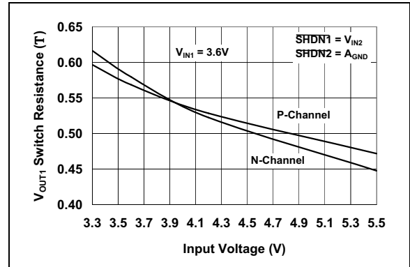
FIGURE 2-16: V_{OUT1} Switch Resistance vs. Input Voltage.
